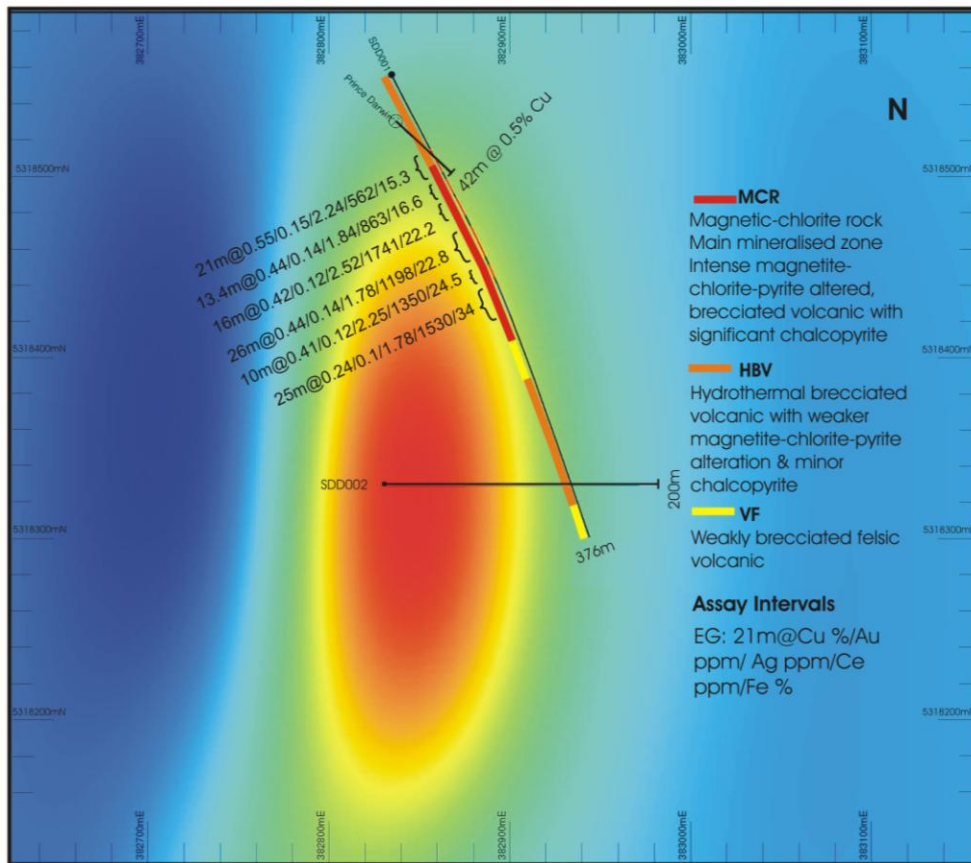
Plan view of SDD001, Prince Darwin adit and magnetic anomaly showing SDD001 skimmed the northern end of the main magnetic anomaly
