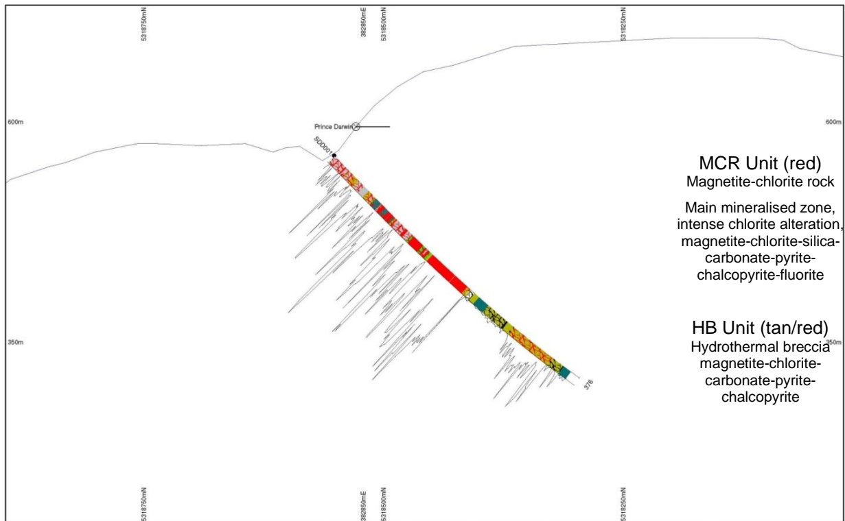
Cross section showing location of SD001 (with magnetic susceptibility and lithology) and historic Prince Darwin adit
