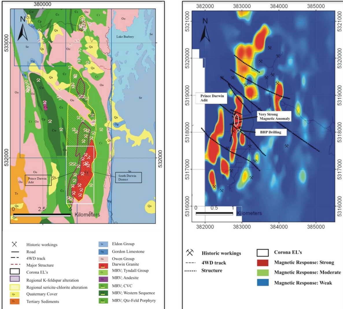
Geology (left) and magnetic image (right) of the South Darwin area. Note numerous magnetic high targets along strike from the current drill area.
