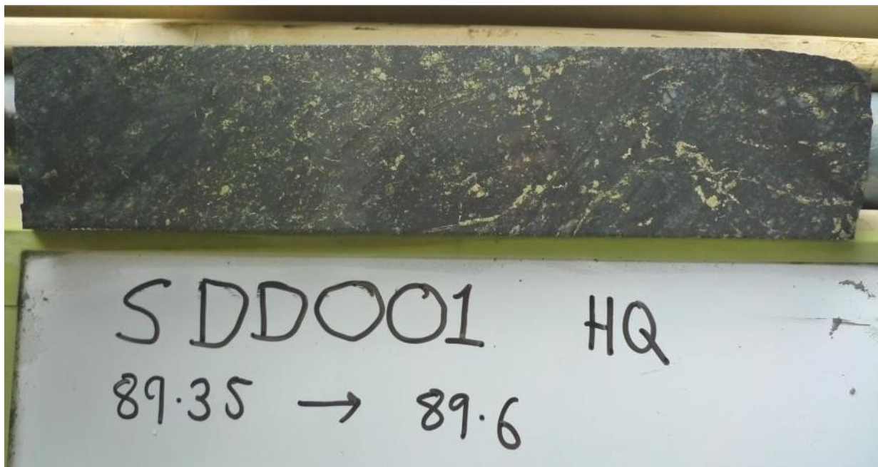
Core sample from SDD001 showing magnetite, chalcopyrite and pyrite mineralisation
